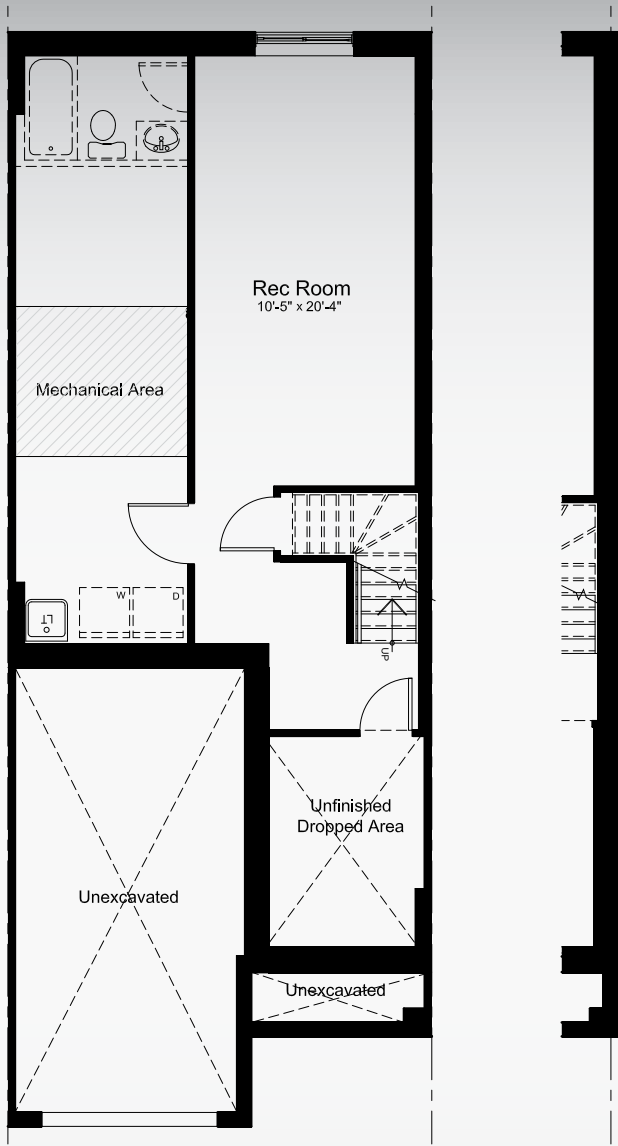
BASEMENT FLOOR
