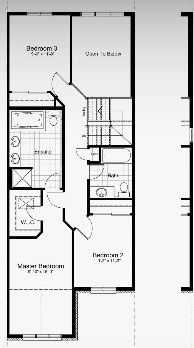
SECOND FLOOR
