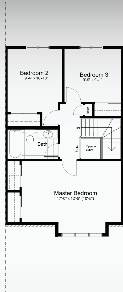
SECOND FLOOR
